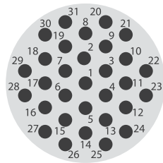
31 x size 16
