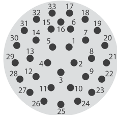
33 x size 20
