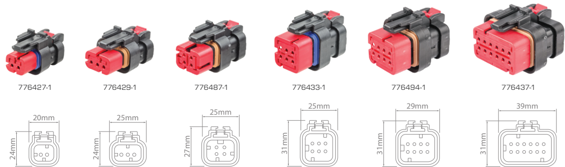
Plugs (Socket Housing)
