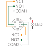
Double Pole
